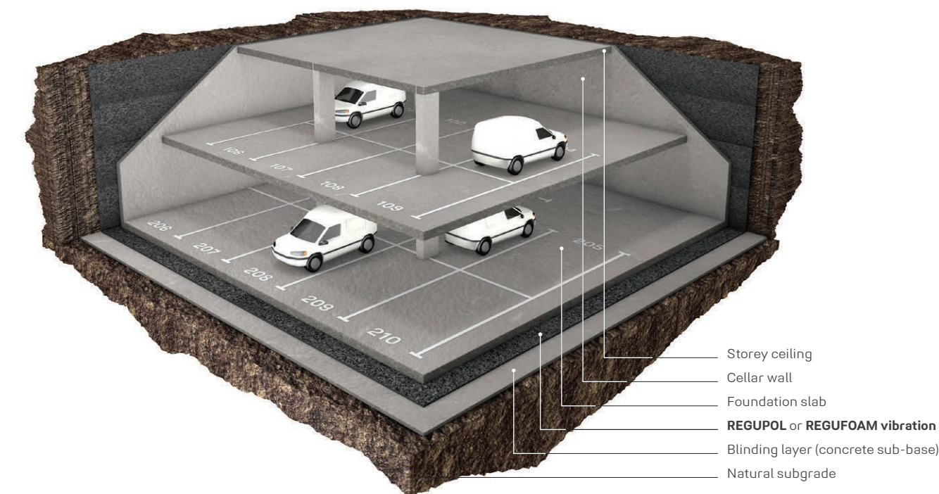
REGUPOL vibration
