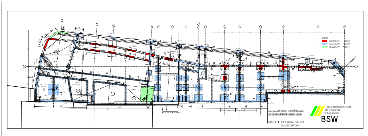
Red: Regupol® MF , green: Regupol® XHT , blue: Regupol® HT
