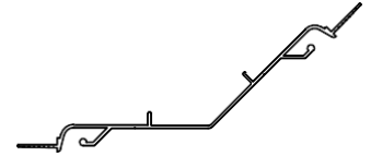
FS-10MN ALUMINUM RETAINER 1/2" DRYWALL (24A162000) 5/8" DRYWALL (24A168000) (SEE SECTION ON PAGE 2 IF WALL IS AN ANGLE OTHER THAN 135°)
