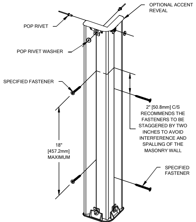
CONCRETE/ C.M.U. WALL APPLICATION
